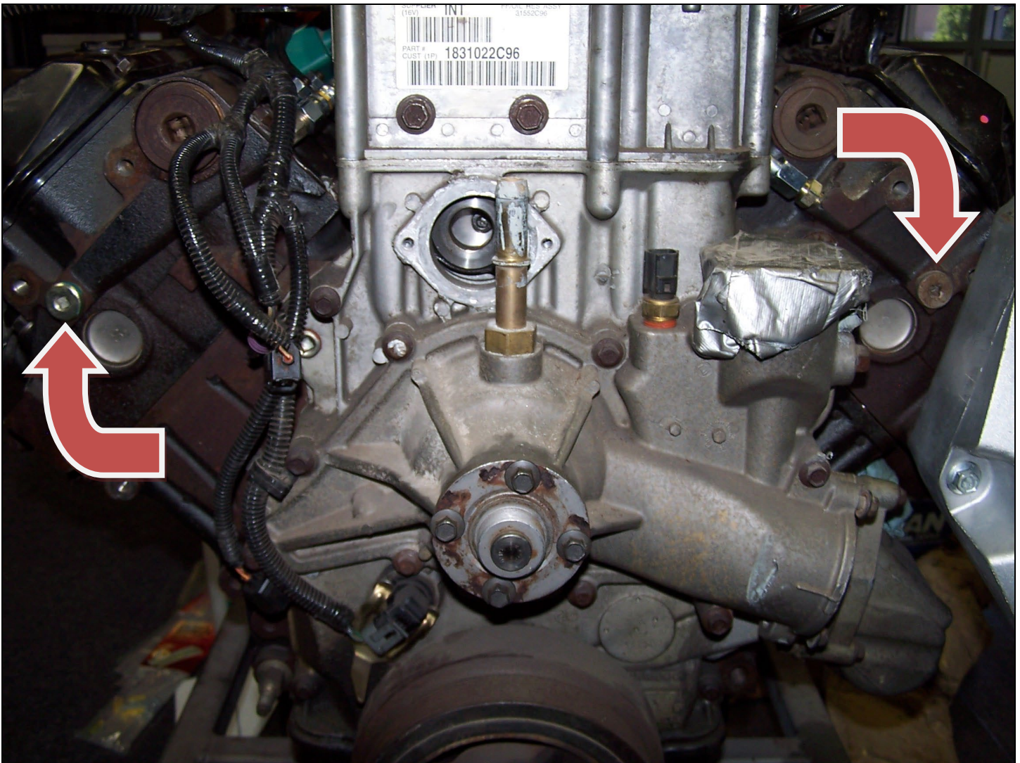
Front of Engine – Arrows Indicate Banjo Bolt Locations
