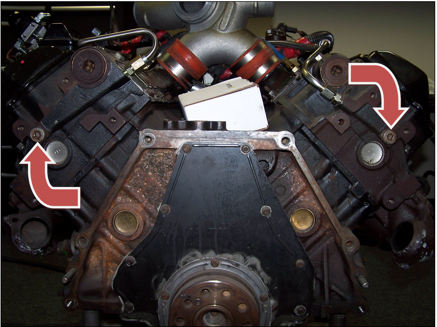
Rear of Engine – Arrows Indicate Banjo Bolt Locations
