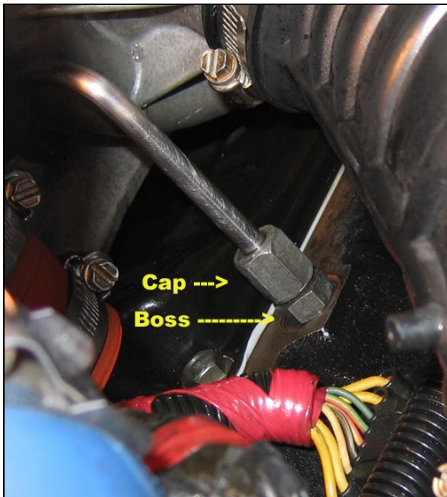
Figure 4 – HPX Line Installed (Driver Side Shown)
